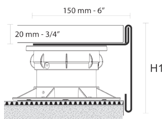
TOP PROFILE PROSUPPORT B - VARNISHED ALUMINIUM length 2,7 lm
