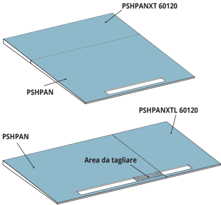
PROSHOWER PANEL EXTENSION VERLEGESHEMA
