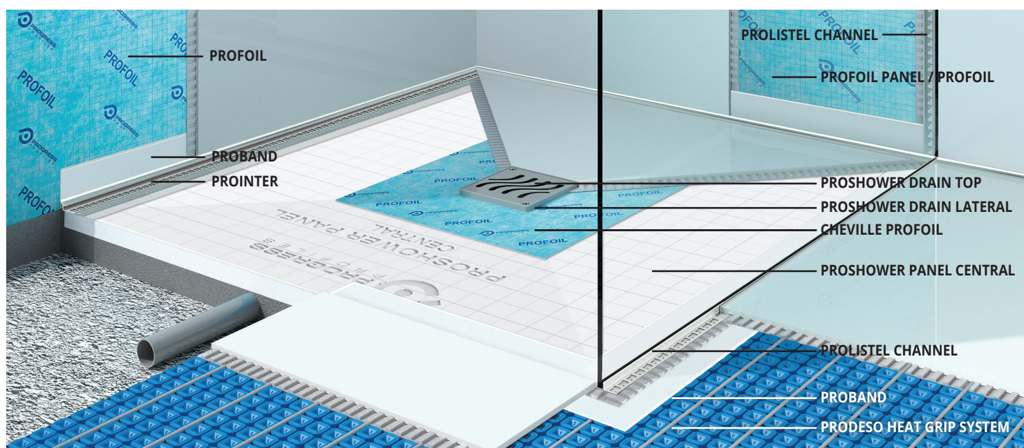
PROSHOWER DRAIN LATERAL KIT PSHLDK
