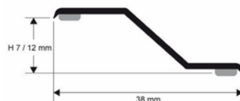
PFRAC 712A/7128AS/7129AS/71210AS/71216AS
