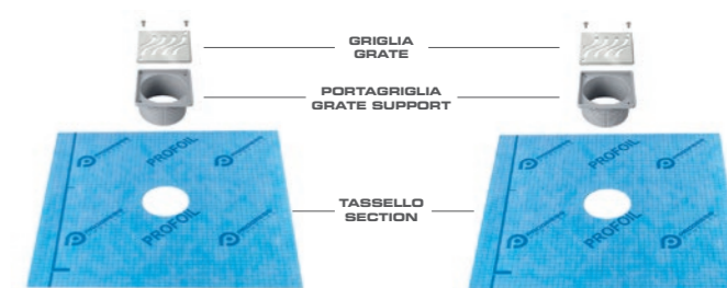
GRIGLIA GRATE PORTAGRIGLIA GRATE SUPPORT TASSELLO SECTION BUTILE BUTYL TAPPO CAP SIFONE SIPHON PROSHOWER DRAIN LATERAL/VERTICAL KIT
